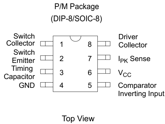
Figure 2. Pin Configuration of BP34063
