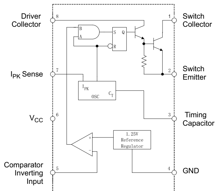
Figure 3. Functional Block Diagram of BP34063
