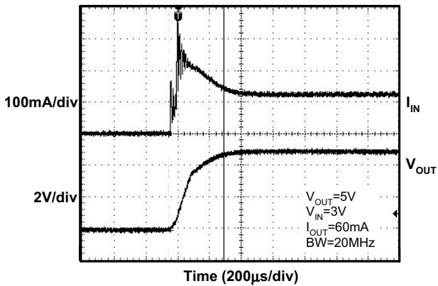
Input Current at Turn-On
