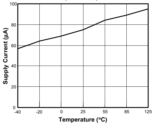
Supply Current vs Temperature (No Load)
